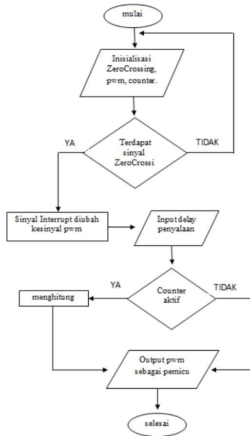
Gbr.9 Flowchart program alat
